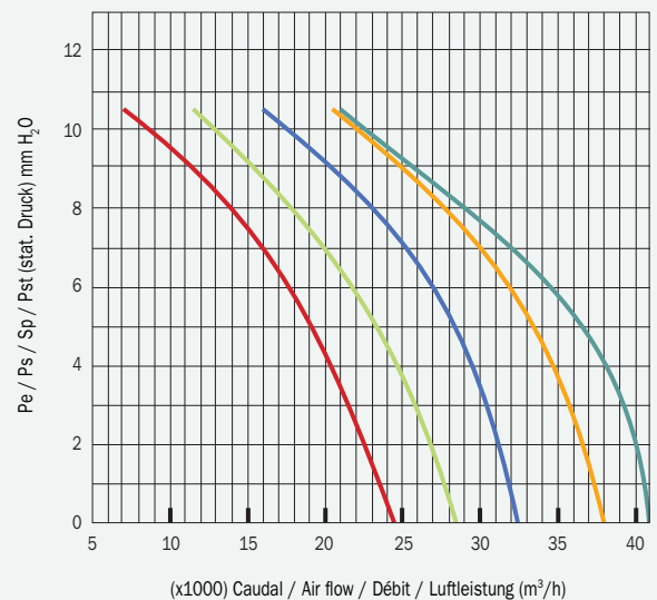
AXIAL SOLID / AXI BOX SOLID / AXITUB SOLID / AXIAN PIROS / AXITUB PIROS / PIROS BOX 700 RPM Ø 1000
