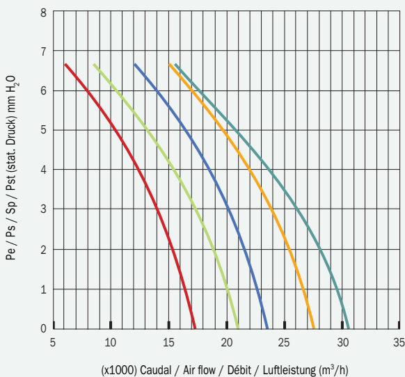
AXIAN SOLID / AXI BOX SOLID / AXITUB SOLID / AXIAN PIROS / AXITUB PIROS / PIROS BOX 700 RPM Ø 900
