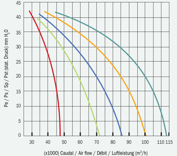
AXIAN SOLID / AXI BOX SOLID / AXITUB SOLID / AXIAN PIROS / AXITUB PIROS / PIROS BOX 900 RPM Ø 1250
